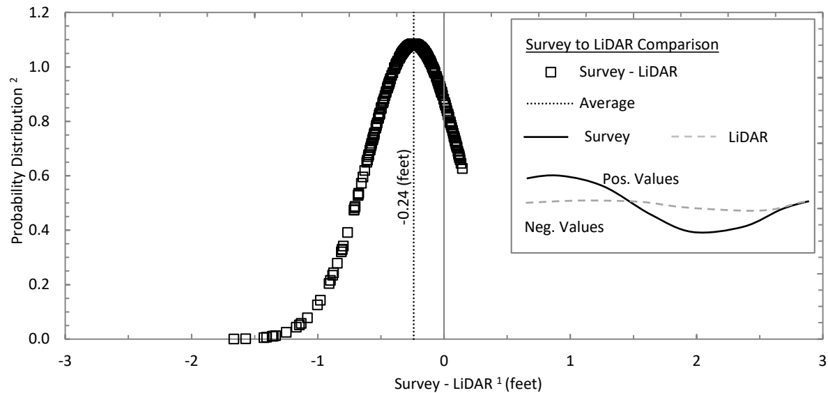
Figure 26: Survey comparison to LiDAR ground elevations.
